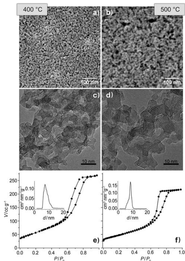
Figure 2. Morphology and crystallinity of nanosized spinel lithium titanate heated at 400 °C (a, c, e) and 500 °C (b, d, f): First row: SEM top view of the films on the FTO substrate; second row: HR-TEM images; third row: nitrogen sorption isotherms with pore size distributions.
