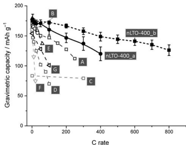
Figure 4. Rate capability of the nano-LTO-400 sample in comparison to previously reported fast LTO materials. mesoporous LTO (A, \square [7d] and B, \circ ), [8] composite LTO-carbon-nanofiber material (C, \square ; the gravimetric capacity is calculated per total mass of the electrode material containing about 50% carbon), [7h] LTO nanoparticles synthesized by the combustion method (D, \square ), [15] LTO prepared by a solvothermal method (E, \triangle ), [7f] surface-modified LTO nanoparticles (F, \nabla ), [7a] LTO/reduced graphite oxide nano-hybrid material (G, \nabla ). [10] The materials cited above can have different thicknesses. Samples nLTO-400_a and nLTO-400_b denote the films with thickness of about 500 nm and 150 nm, respectively.
